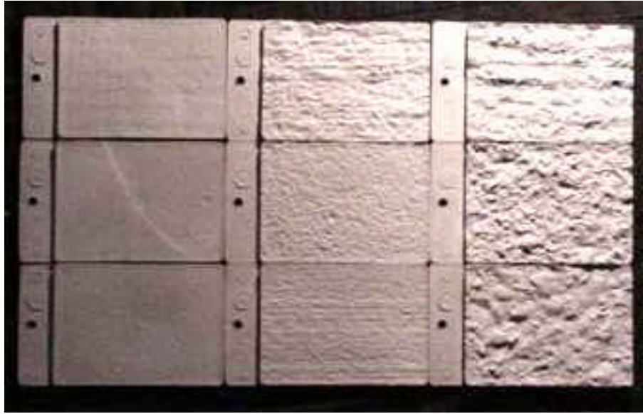
Figure 3: Plastic model concrete surface profiles. The profiles are ordered 1 to 9 in order of increasing roughness, and correspond to acid etching, grinding, light shotblast, light scarification, medium shotblast, medium scarification, heavy abrasive blast, scabbing, and heavy scarification.
