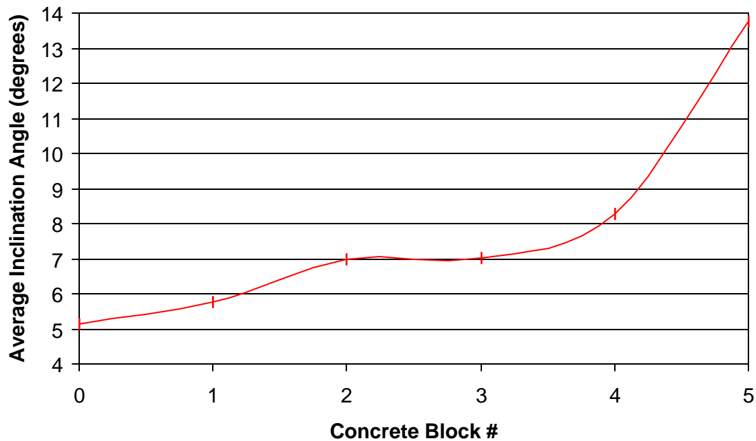
Figure 10. Roughness measurement results for the 6 concrete surfaces in terms of the average inclination angle of the profiles.
