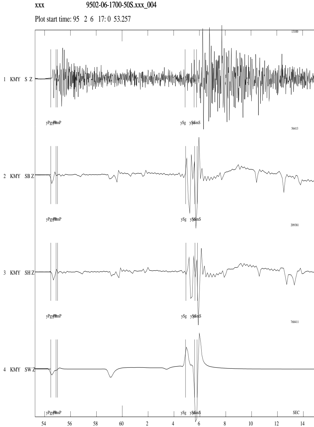
Figure 7.34: An example of synthetic seismograms using Bouchon(2), Herrmann (3) and WKB(4). The original seismogram is shown in channel 1. All synthetics are displacement. Also shown are the theoretical travel times calculated by WKB.
