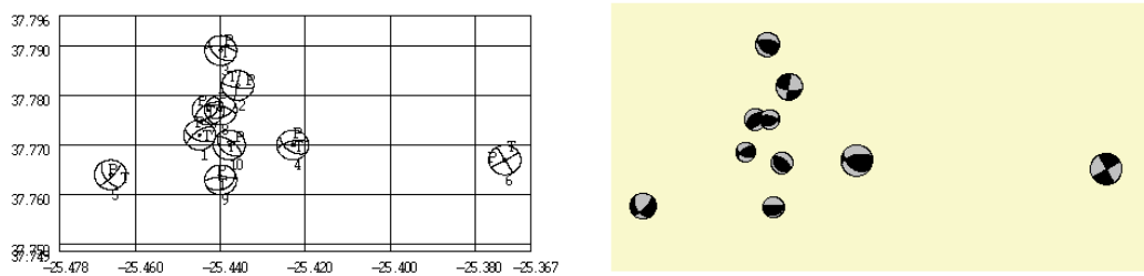
Figure 7.28: Plotting many fault plane solutions. Left: Using WEMAP. Notice that the colors in the solutions are inverted compared to normal practice. Right: Using EPIMAP. The data for the two plots is the same.
