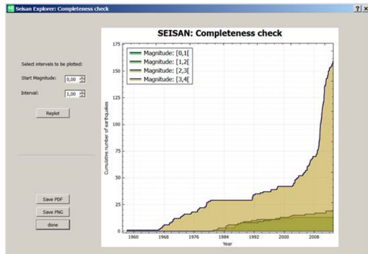
Figure 4.9: se-completeness
