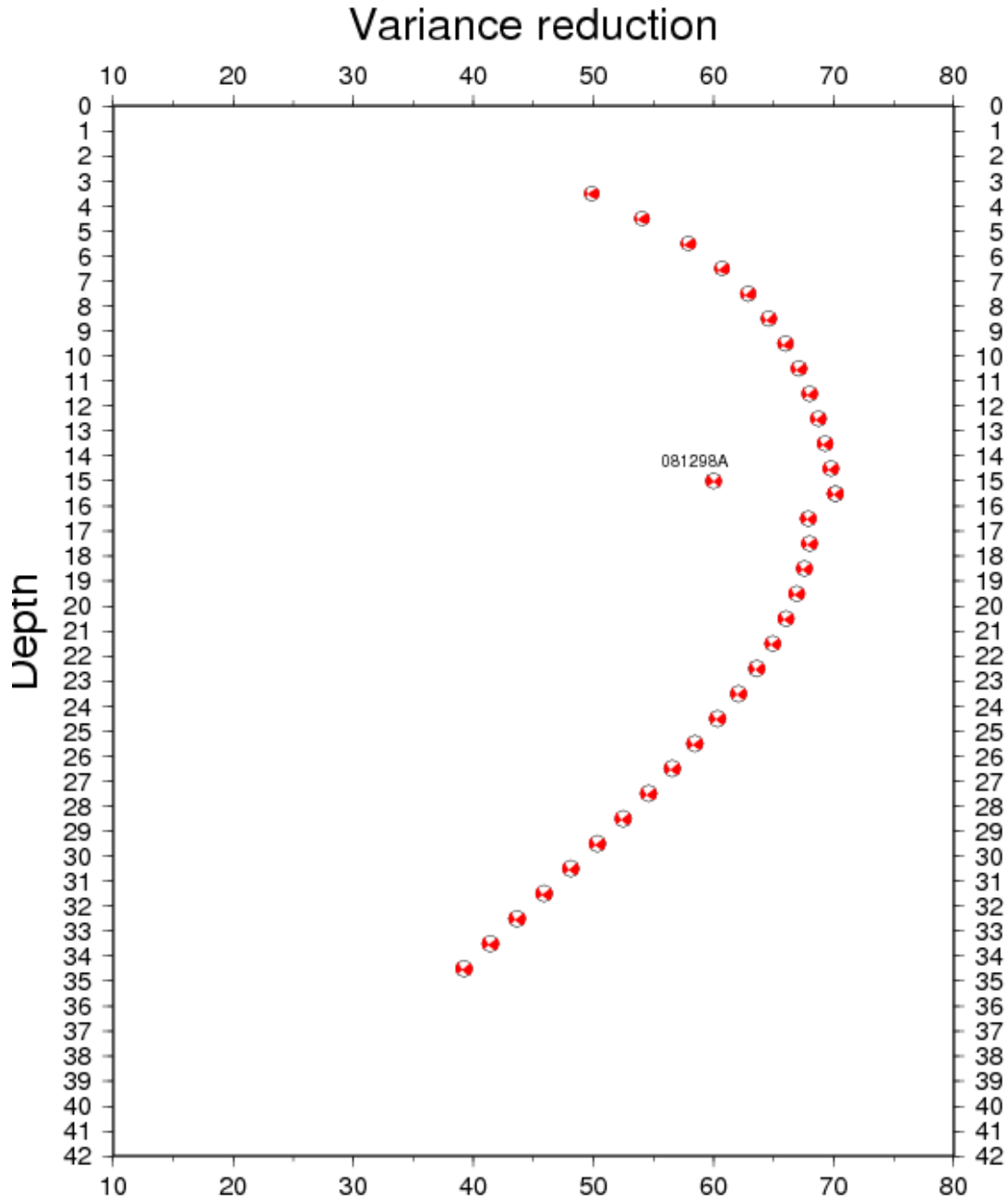
Figure 7.32: The double couple part of the moment tensor solution shown with respect to the variance reduction at different depths. The GCMT solution is also shown with arbitrary variance reduction. This figure was made with the GMT program psmeca , see text.
