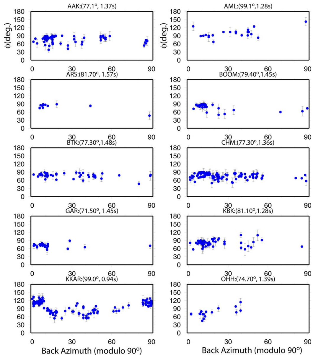
Figure 6. Azimuthal variations of observed fast orientations for each of the Group 1 stations. Values in the parentheses following the station name are station-averaged fast orientation and splitting time.
