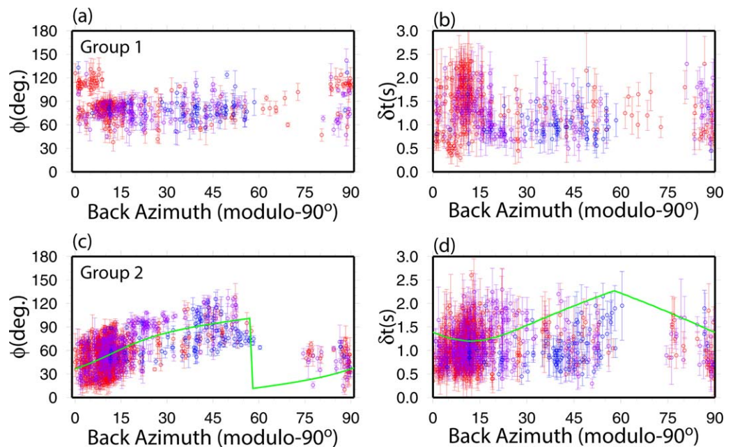
Figure 5. Azimuthal variations of all of the resulting SWS parameters plotted against modulo-90° BAZ. (a and b) are measurements from Group 1 stations, and (c and d) are those from Group 2 stations. Red, purple, and blue symbols are SKS, SKKS, and PKS measurements, respectively. The solid line in Figures 5c and 5d are theoretical apparent splitting parameters computed using a nominal period of 5 s and \phi = -65^\circ and \delta t = 1.7 s for the lower layer, and \phi = 77^\circ and \delta t = 1.4 s for the upper layer.
